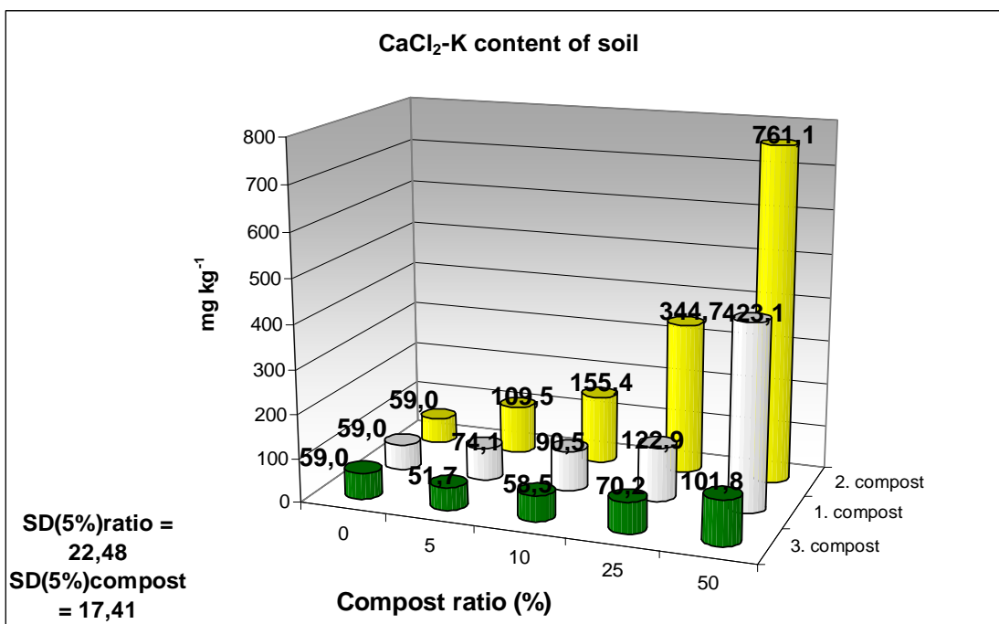
Fig. 4 The 0.01 M dm -3 CaCl 2 extractable K content of soil
