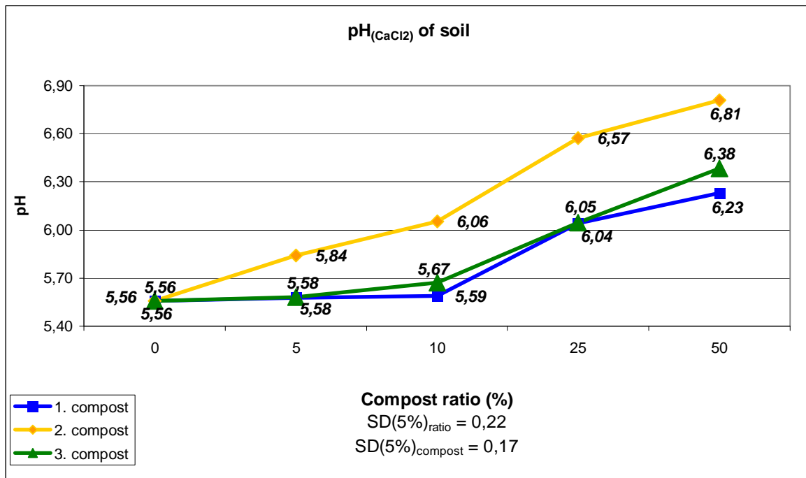
Fig. 6 pH(CaCl 2 ) of soil
