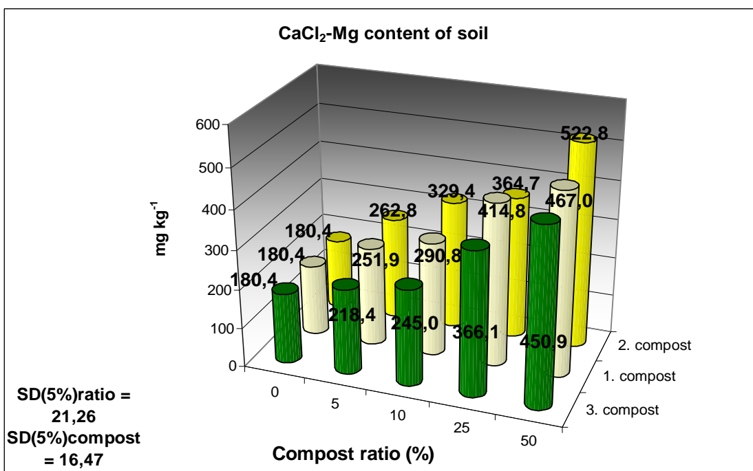
Fig. 5 The 0.01 M dm -3 CaCl 2 extractable Mg content of soil
